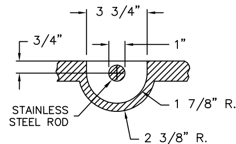
(2) TYPE 4 STEEL PICKBARS PICKBAR DETAIL
